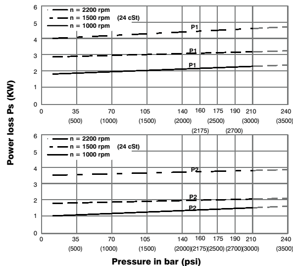
HYDROMECHANICAL POWER LOSS (TYPICAL)
