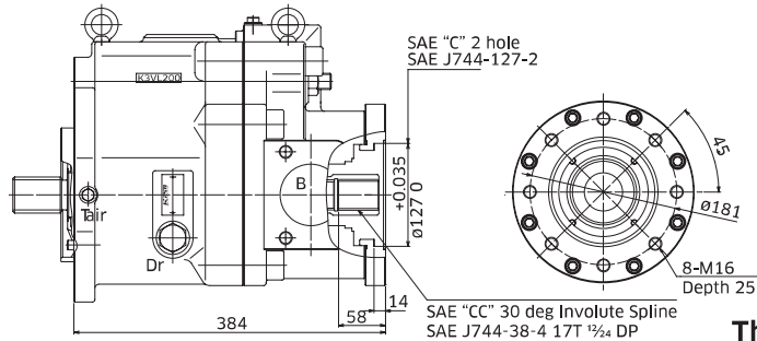
Through Drive 'CC'
