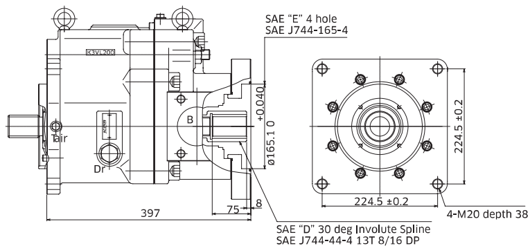
Through Drive 'E'
