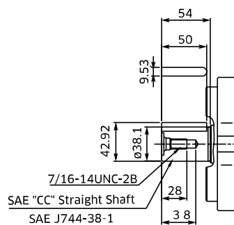
SAE 'CC' Straight Shaft - Option 'Y'
