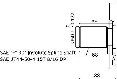
SAE 'F' Spline Shaft - Option 'F'
