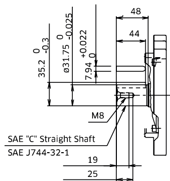
SAE 'C' Straight Shaft - Option 'X'
