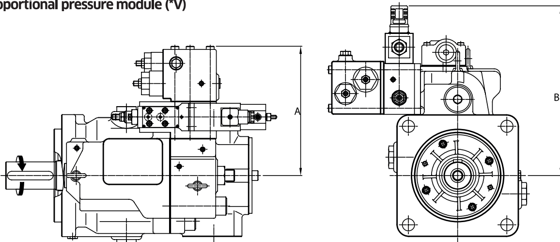
Proportional pressure module (*V)
