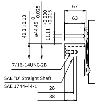
SAE 'D' Straight Shaft - Option 'K'
