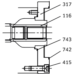
SAE 'C' & 'C4' T/D KIT
