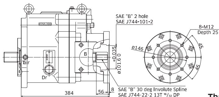
Through Drive 'B'
