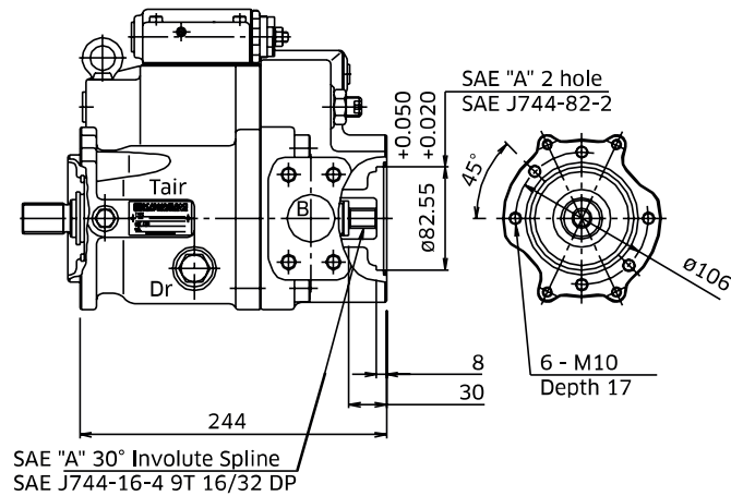
Through Drive 'A'
