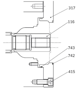
SAE "BB" T/D Kit
