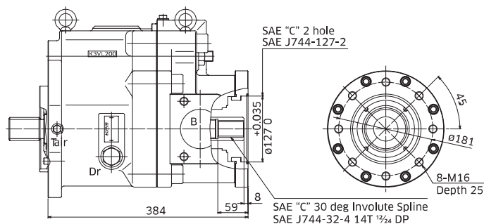
Through Drive 'C'
