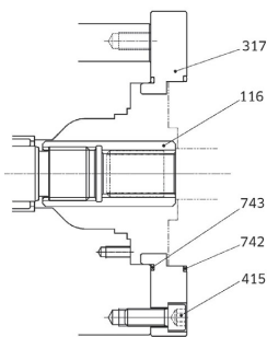
SAE "C" & "C4" T/D Kit
