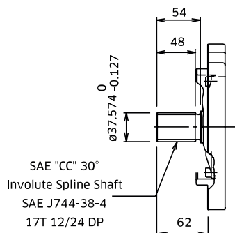
SAE 'CC' Spline Shaft - Option 'W' & 'T'
