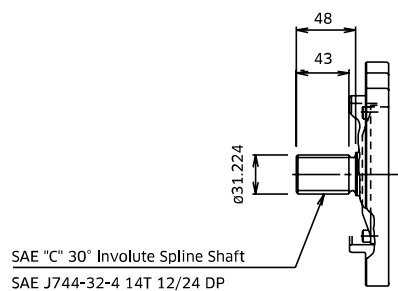
SAE 'C' Spline Shaft - Option 'S'
