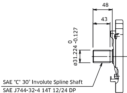
SAE 'C' Spline Shaft - Option 'C' & 'R'
