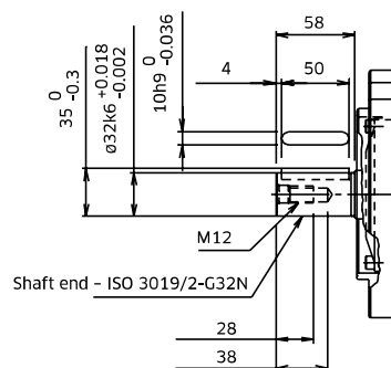
ISO Straight Shaft - Option 'M'
