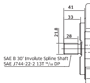
Model Code Option 'S' Shaft
