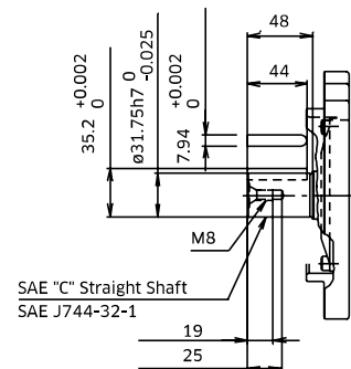
SAE 'C' Straight Shaft - Option 'K'
