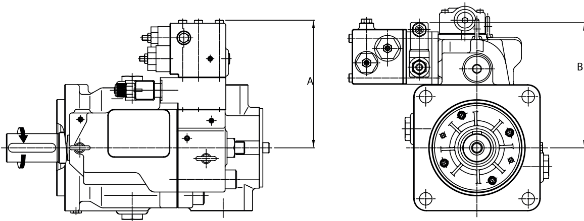
Proportional pressure module (*V)
