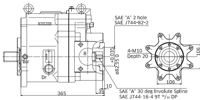
Through Drive 'A'
